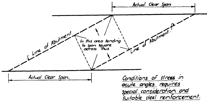
PLAN OF SKEW BRIDGE.
